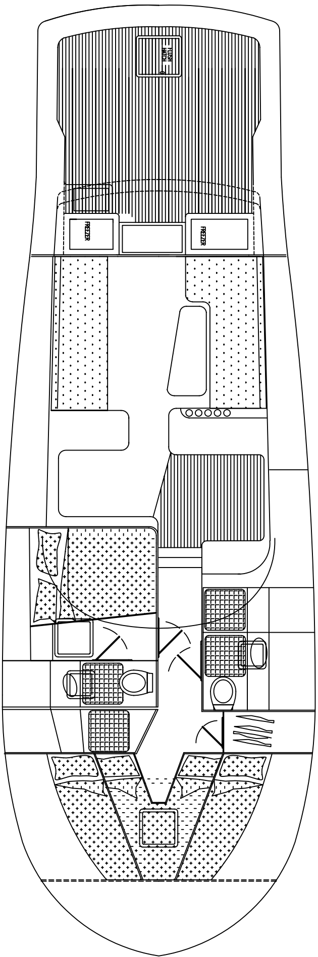
PLAN ON DECK
